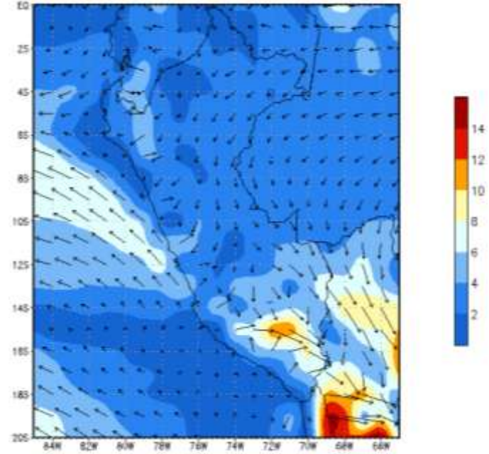
otachs (m/s) 850 mb Tue 18Z 25jun2013
